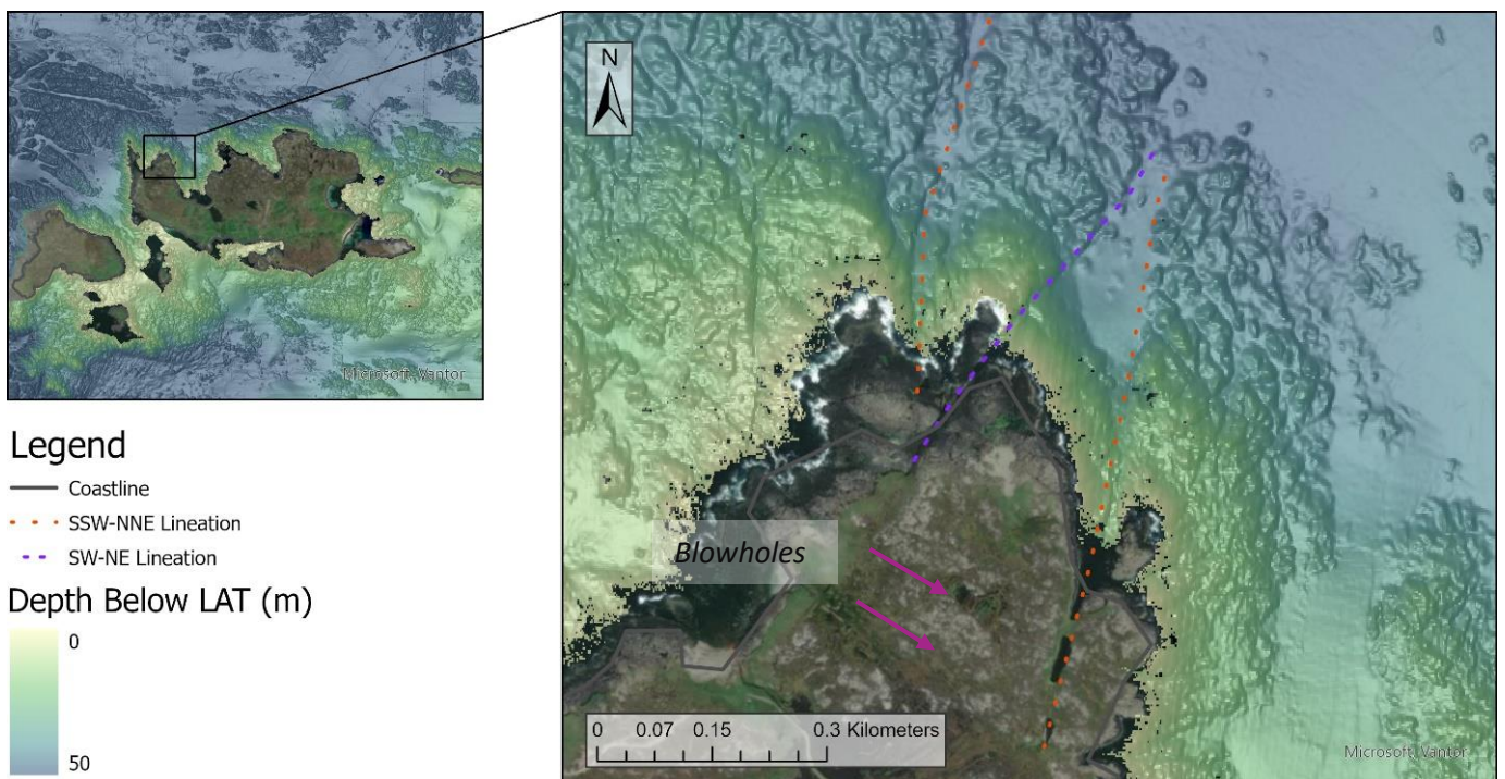
Figure 10: Bathymetry around the blowholes showing a south-south-west to north-north-east oriented seabed lineation aligned with their orientation.
