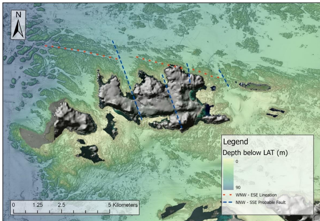
Figure 11: Bathymetry showing a large west-north-west to east-south-east lineation, possibly offset by north-north-west to south-south-east lineaments.
