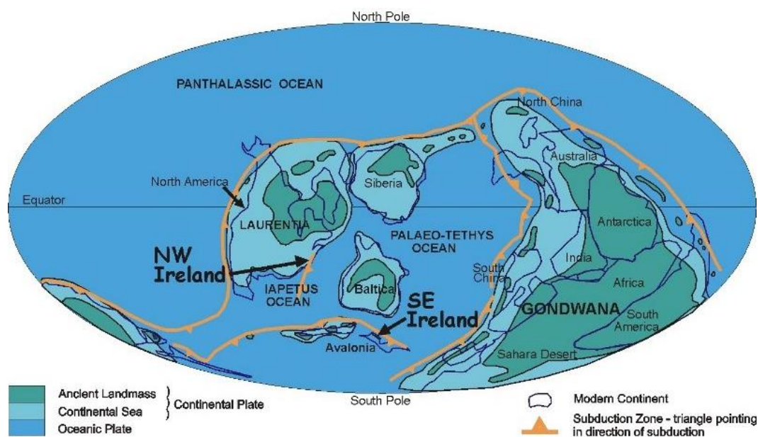
Figure 2: Palaeogeography of Ireland at the beginning of the Ordovician period. Image from (Geological Survey Ireland, n.d.).
