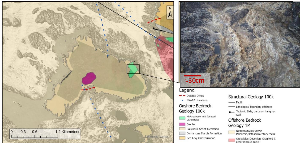
Figure 20: Geology of Inishark, with image of exposed talc on the north-east shore from (Meehan, et al., 2019).
