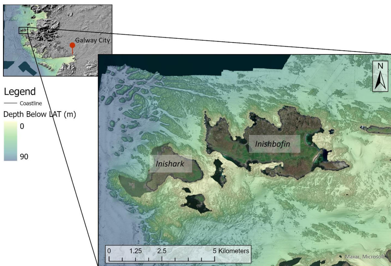
Figure 1: Bathymetry of the seabed around Inishbofin and Inishark. Depths are referenced to Lowest Astronomical Tide (LAT).
