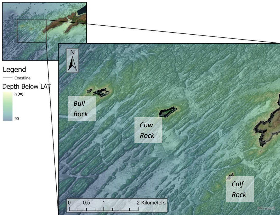
Figure 9: Bathymetry surrounding the Calf, Cow and Bull Rock.
